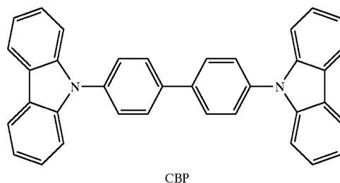
Structural formula (3)
