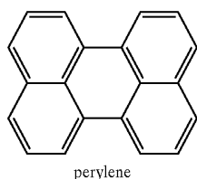
perylene
