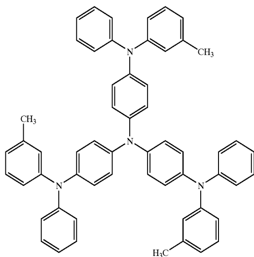
Structural formula (4)
