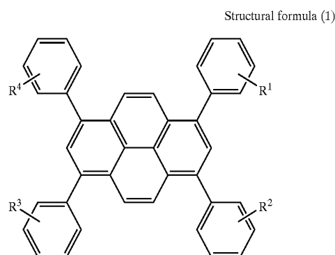
Structural formula (1)
